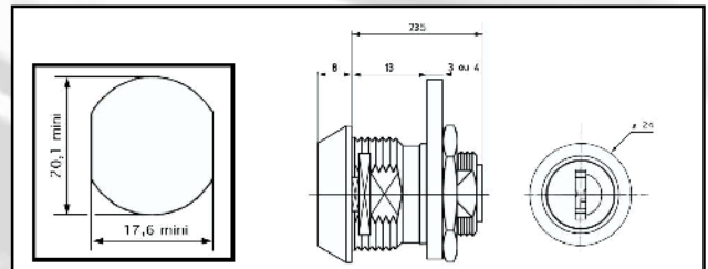
BAT-7302-B7B Cam de type S3-S4
